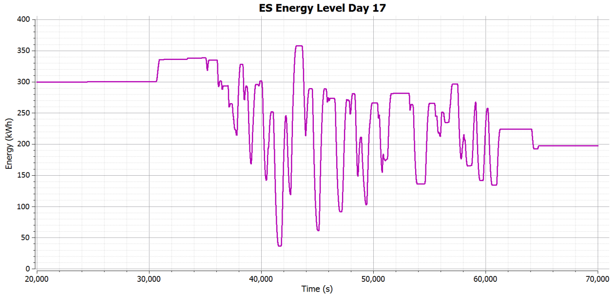
Figure 5-5. Graph that indicates how the energy content, expressed in kWh, would change during day 17. If the BESS would provide this service only this day, it would lose 102 kWh from the morning to the evening.
