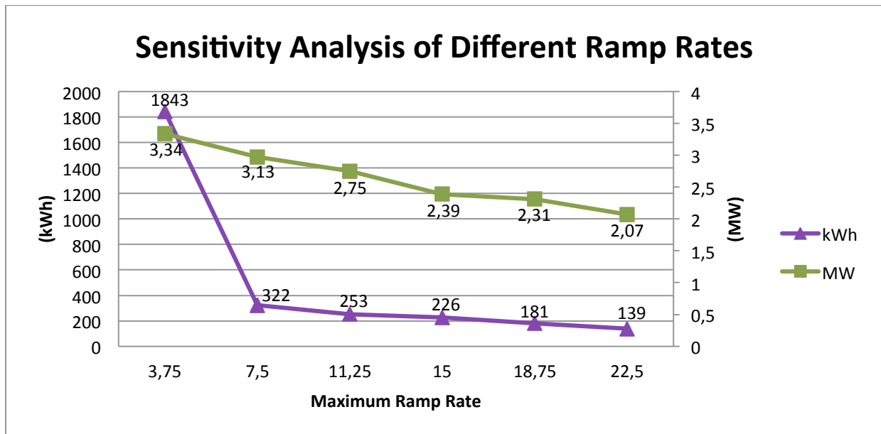
Figure 5-6. Graph showing how the dimensions of the BESS is changing depending on the ramp rate. The green line indicates the required power and is expressed at the right y-axis. The purple line indicates the required energy content and is expressed on the left y-axis.
