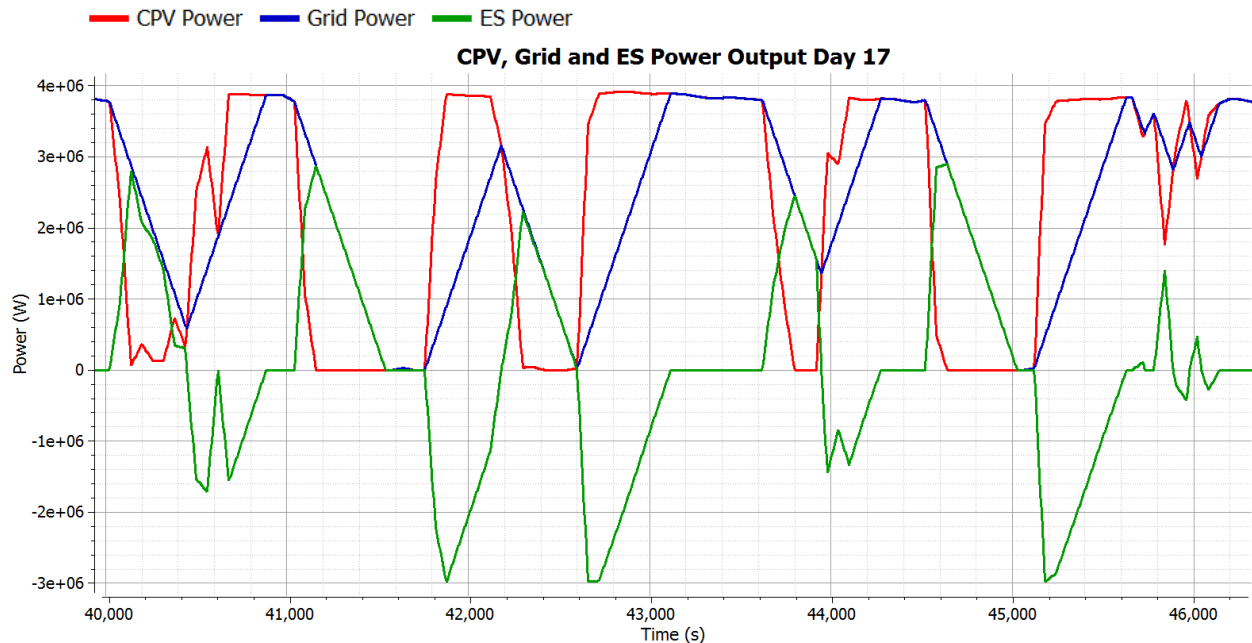
Figure 5-3. Graph describing how the BESS prevent rapid changes in power output to the grid and when the BESS is charging/discharging over a time of 6000 seconds (about 1.5h) during day 17.
