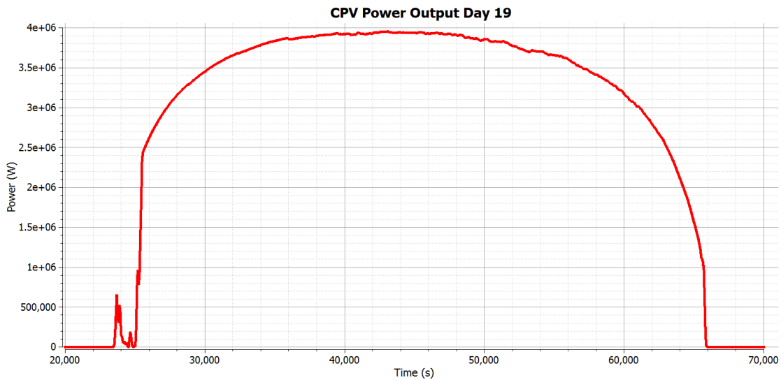
Figure 5-1. Graph describing the power output of September 19 th for a close to perfect sunny day where the y-axis shows power [W] and the x-axis the time [s].
