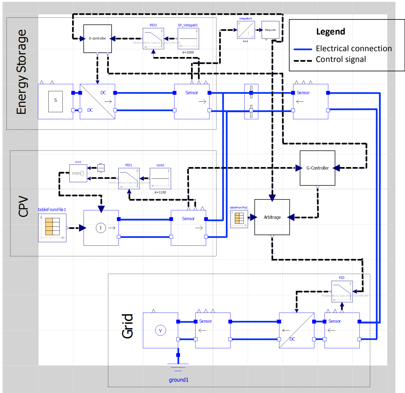
Figure 4-2. Illustration of the model used in OpenModelica for the combination of the three services.
