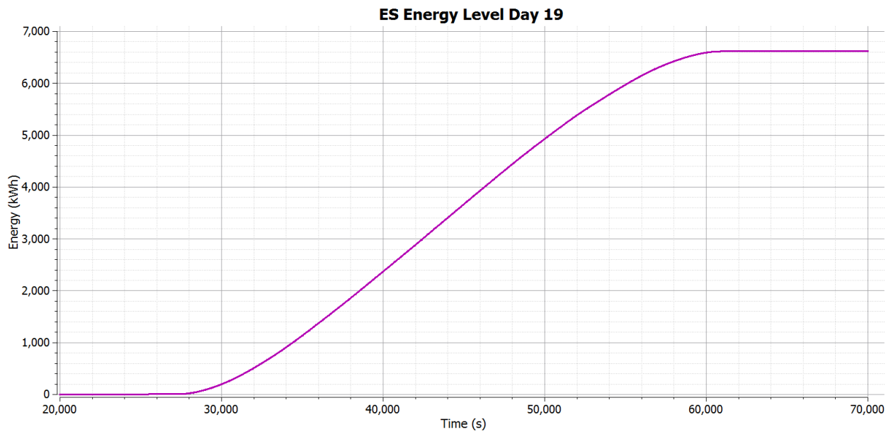
Figure 5-8. Graph shows how the energy rating in the BESS would increase for a sunny day at the SDP without any clouds if the only provided service is to peak shave at 3 MW
