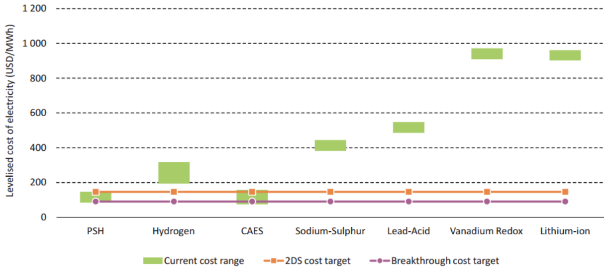
Figure 3-7. The LCOE in current cost range (2013) and breakthrough scenarios until 2050 expressed in USD/MWh (IRENA, 2014).
