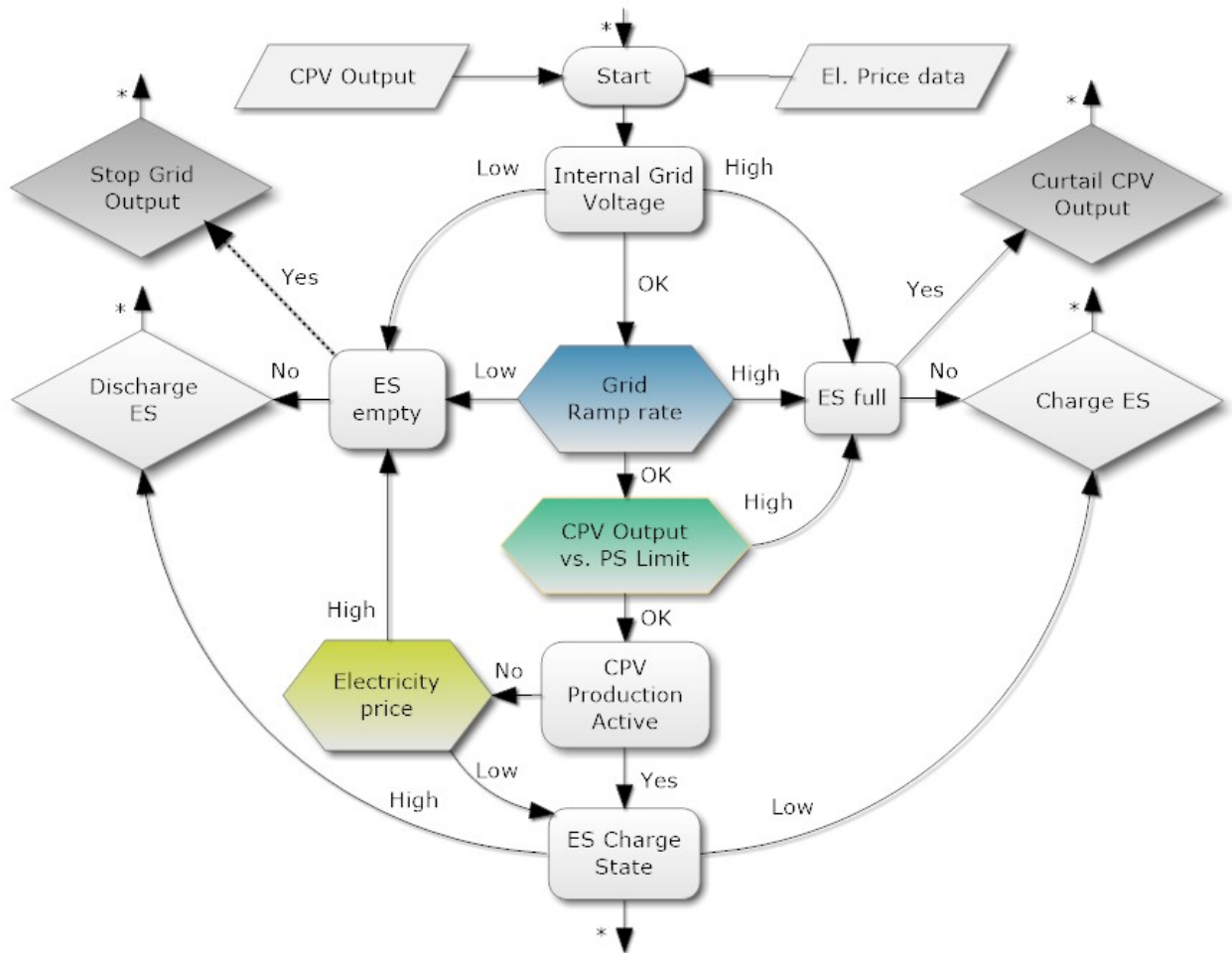
Figure 4-1. Flowchart showing the overview of the BESS control strategy.
