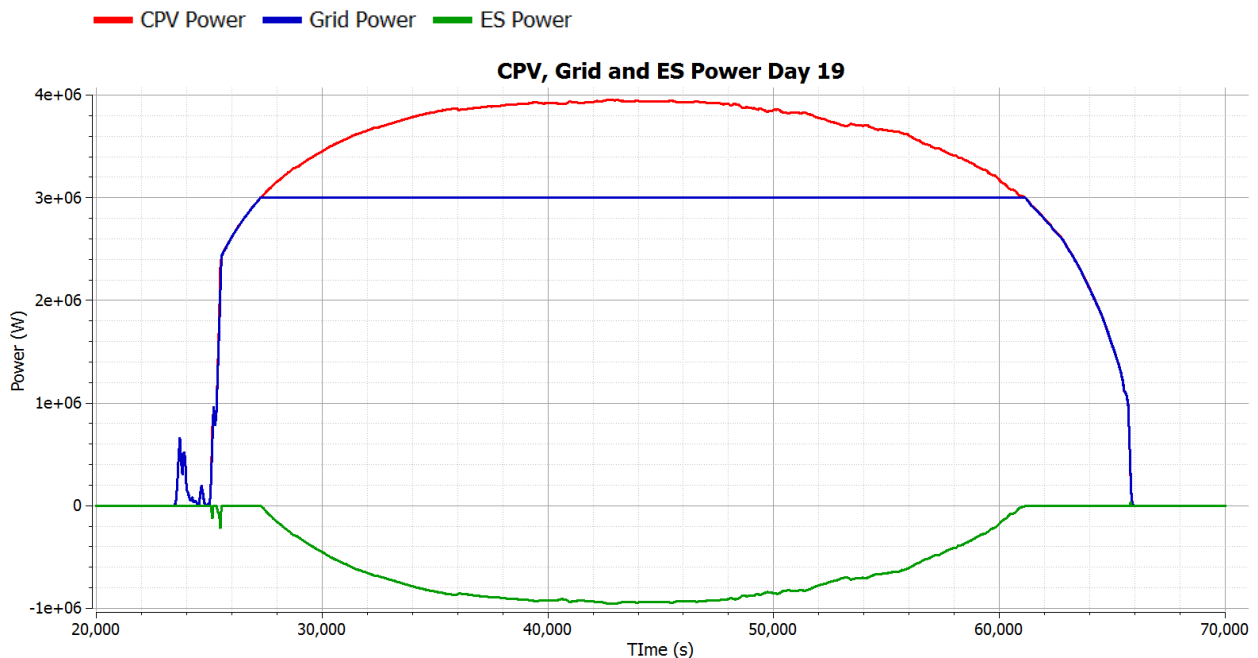
Figure 5-7. Graph demonstrating how the BESS would work if the provided service would be peak shave at 3 MW.
