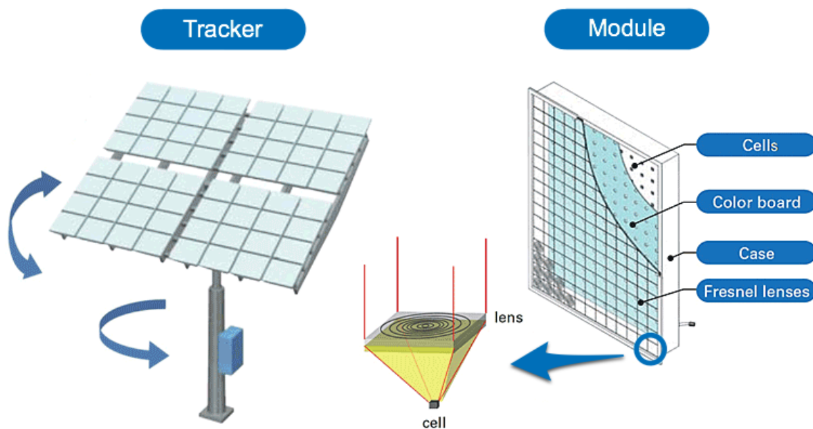
Figure 2-5. Sketch of CPV technology similar to the one used at the SDP (Sumitomo Electric Industries, Ltd., 2014). Picture edited by author.
