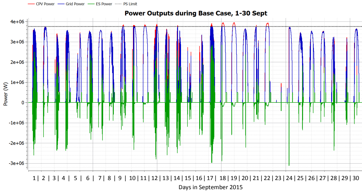
Figure 5-12. The power output [W] from the CPV, the battery and to the grid on the y-axis is plotted from the 1/9 to the 30/9.
