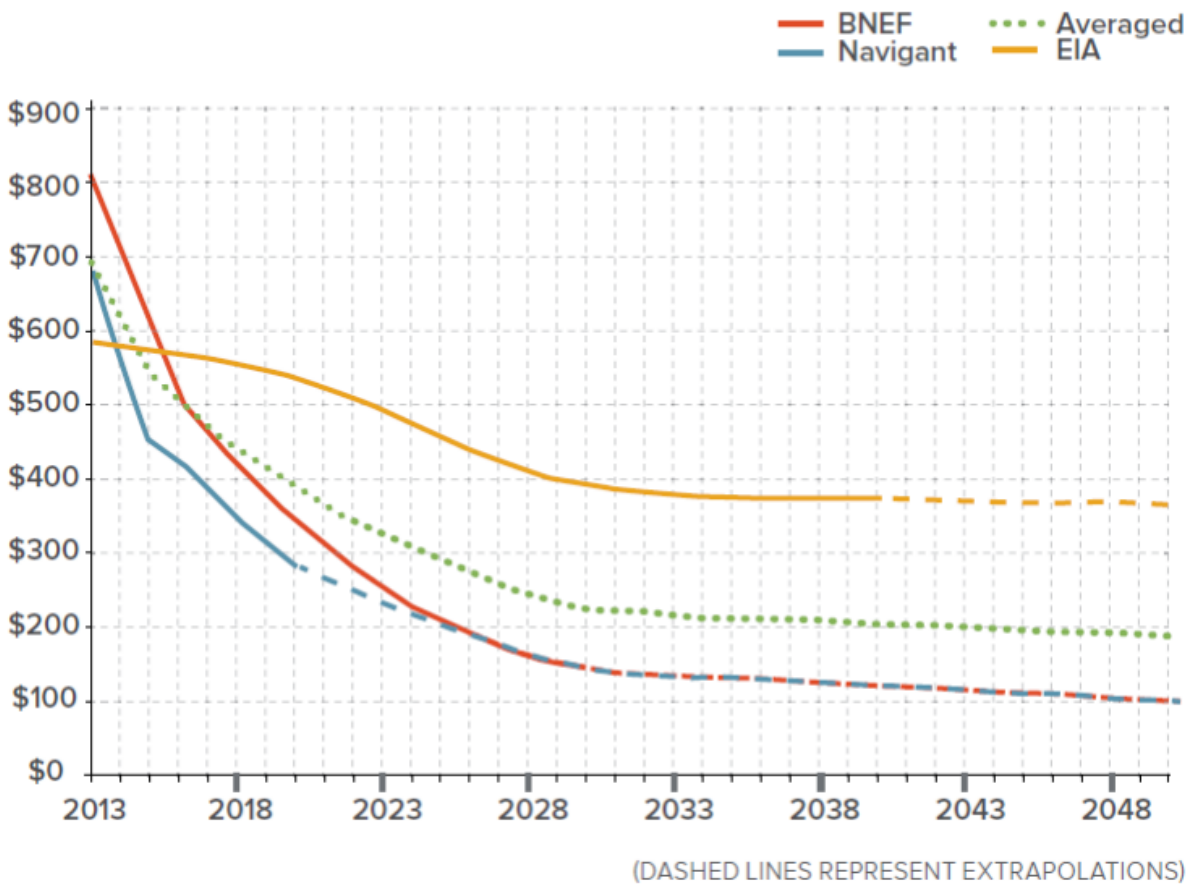
Figure 3-8. Prediction of the cost reduction of BESS in the future according to three sources. Y-axis is USD/kWh 2012 (Deutsche Bank, 2015).
