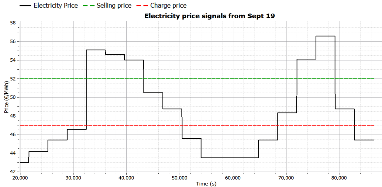
Figure 5-11. Graph showing how the hourly spot market price, expressed in EUR/MWh, is changing during day 19. The green dashed line indicates the minimum selling price and the red dashed line indicate the highest price for the BESS to charge.
