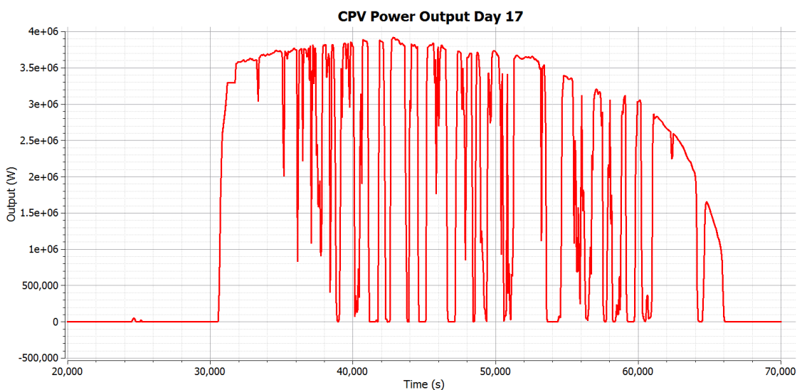
Figure 5-2. Graph describing the power output of September 17 th for a sunny day with many clouds passing by during the day where the y-axis shows power [W] and the x-axis the time [s].
