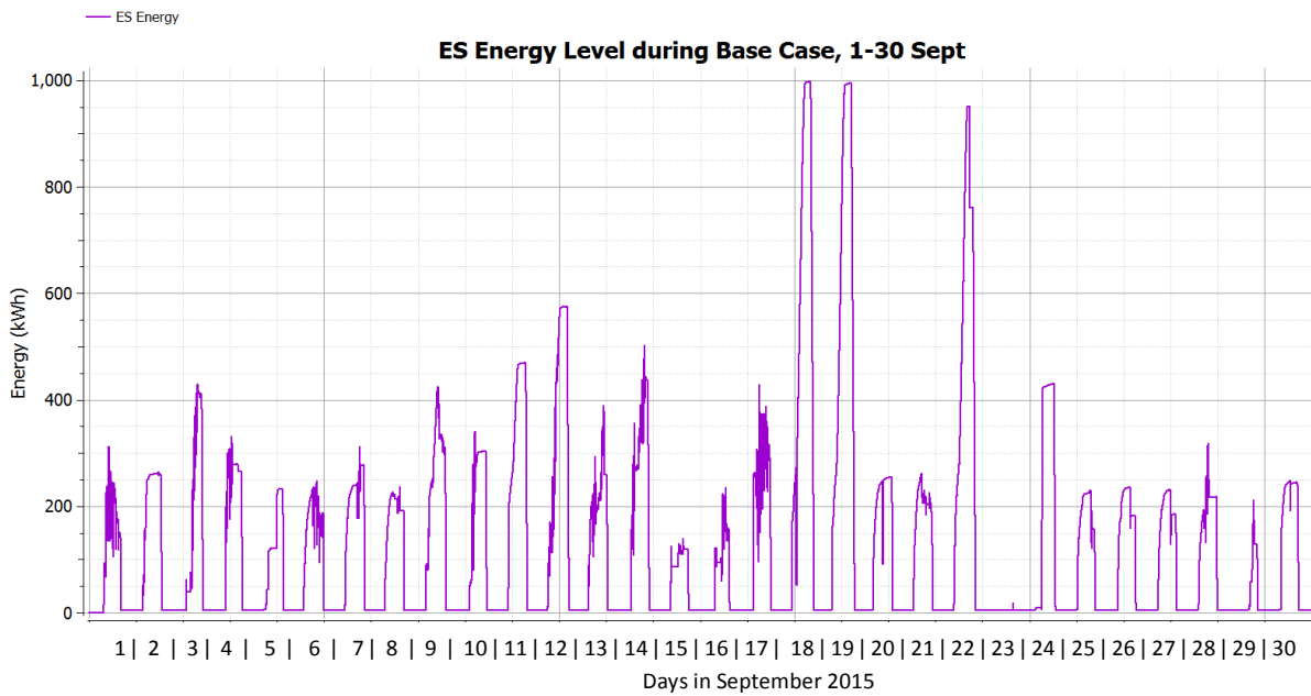
Figure 5-14. The energy content [kWh] of the battery on the y-axis is plotted from the 1/9 to the 30/9.
