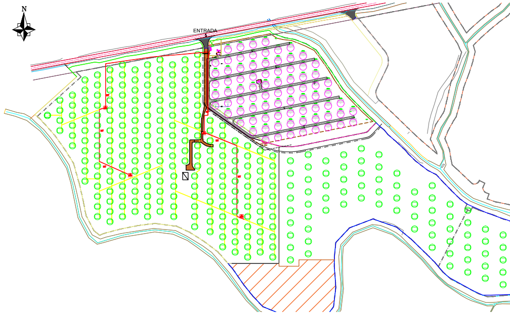
Figure 2-2. Sketch of the SDP with the installed trackers as green and purple circles. The 15 kV voltage level of the internal grid for one of the CPV technologies is shown as red lines (Enercoutim, 2016b).
