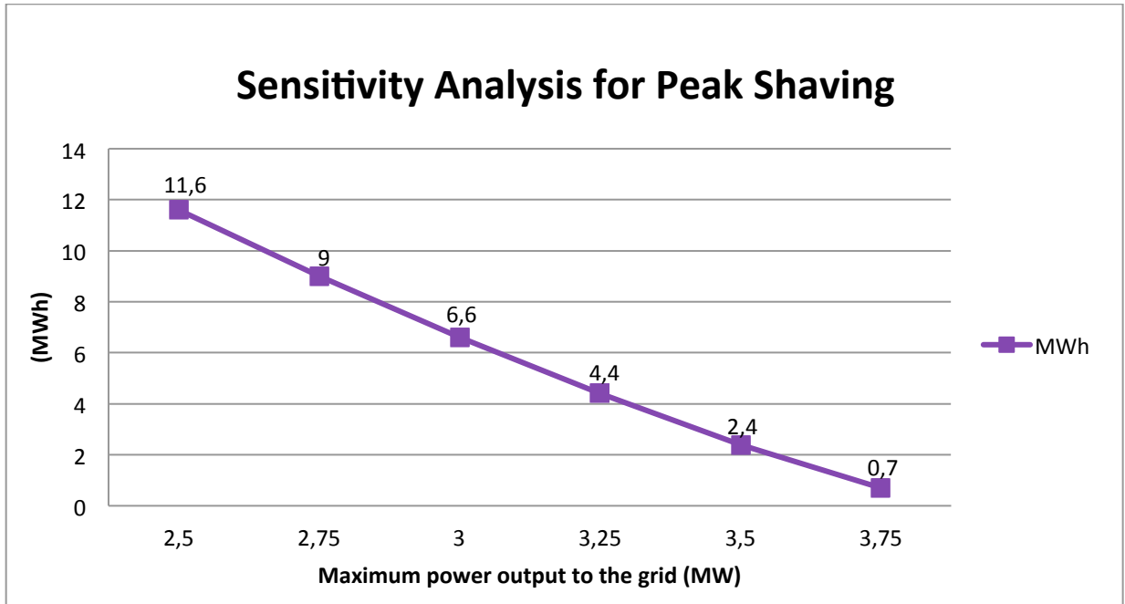
Figure 5-9. Graph showing how much energy the BESS needs to contain in order to guarantee the delivered power to the grid not to exceed a certain value. The maximum power rating to the grid was tested between 2.5 MW to 3.75 MW.
