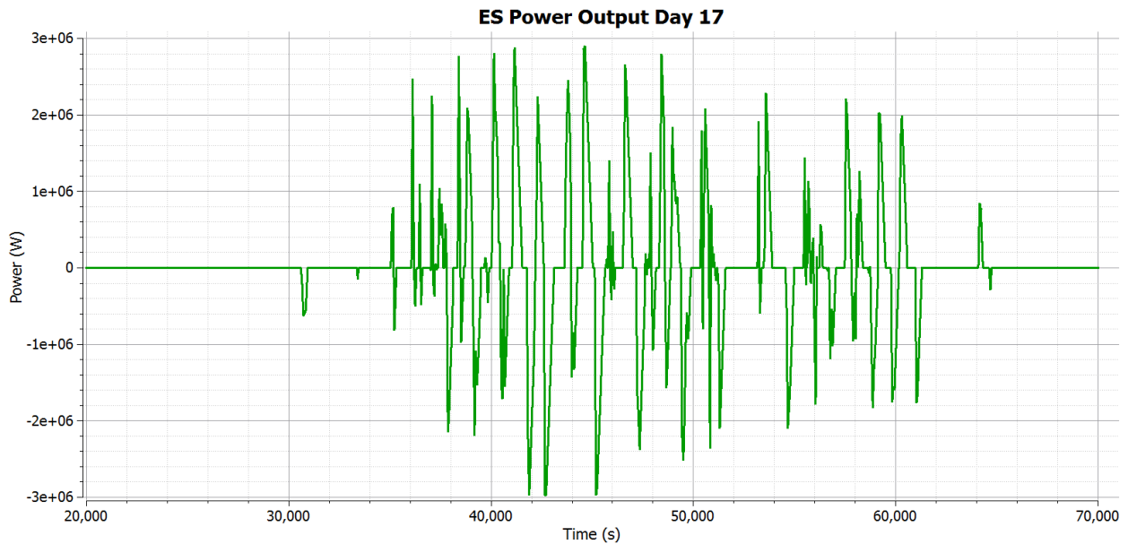
Figure 5-4. Graph showing when the battery is charging and discharging for the whole day 17. The maximum power output/input for this day is 2.97 MW.
