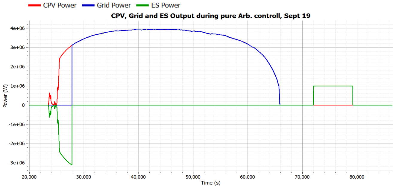
Figure 5-10. Graph that shows how the power profile of the CPV, red line, the power to the grid, blue line, and the BESS when arbitrage is the only service provided. The blue line covers the red line from about 28 000 seconds to 66 000 seconds and the green line covers the blue line from 66 000 seconds to the end of the graph.
