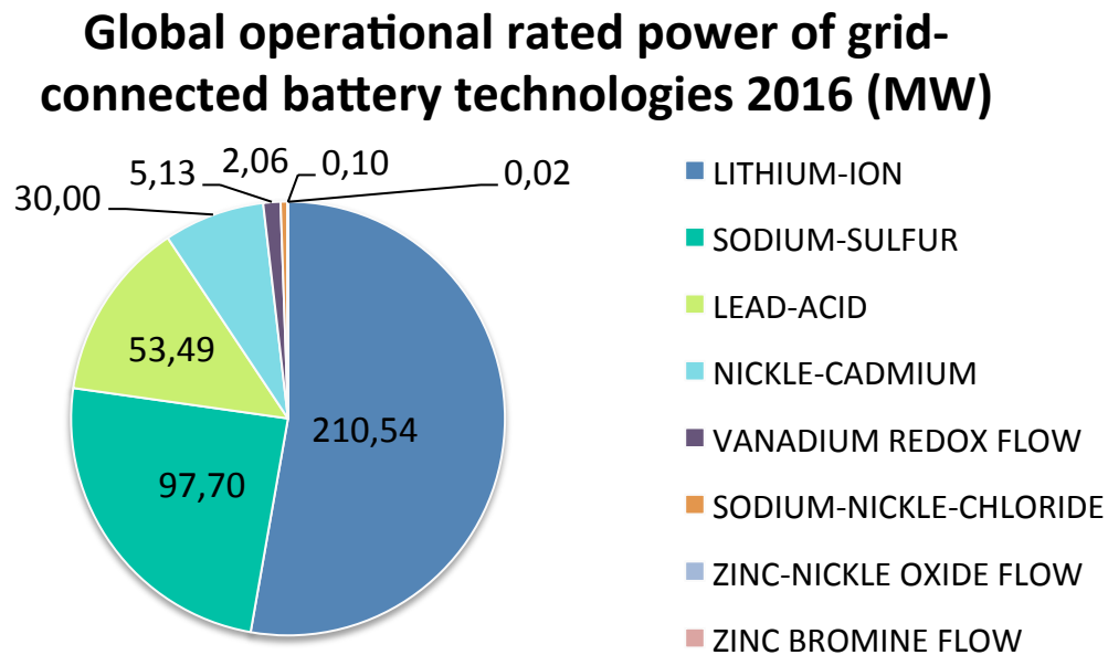
Figure 3-5. Overview of global installed and operational power output of battery technologies 2016 (DOE, 2016c).
