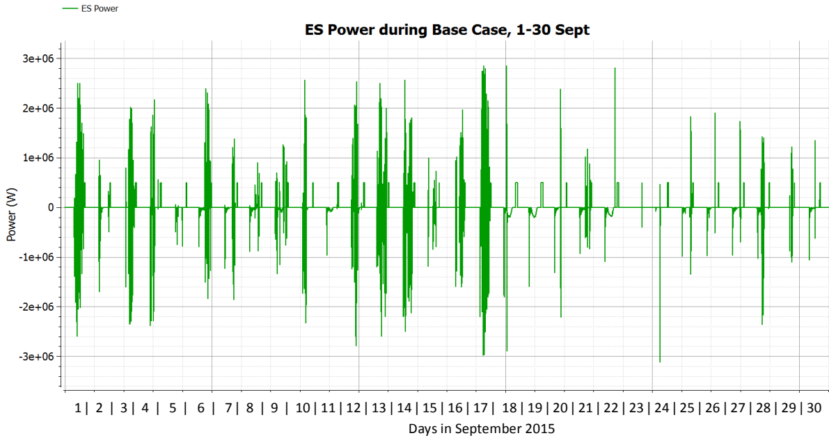
Figure 5-13. Illustration of the power rating requirement of the battery from the 1 st to the 30 th of September.
