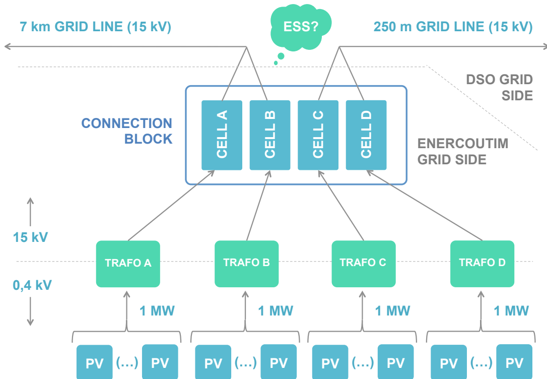
Figure 2-3. Sketch of the system layout, as of the time writing, from the power producing trackers at the bottom, to the DSO export connections on top. Also the suggested level of ESS-to-grid connection is marked out.
